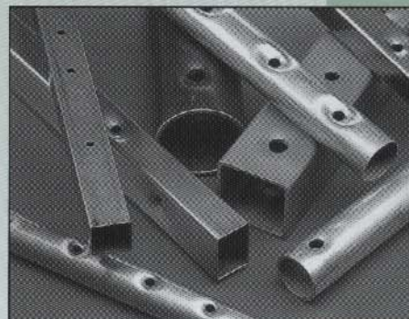
Tube Punching - Round or Square Tubing
