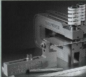
Typical 3-pin gaging Template Mounting
