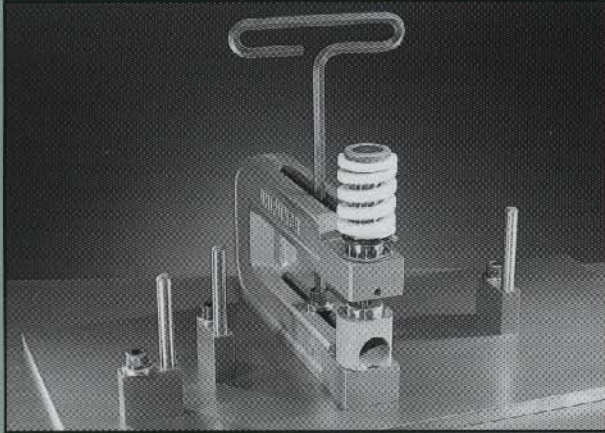
Typical 3-pin gaging Template Mounting
