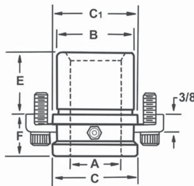
SHORT SHOULDER
