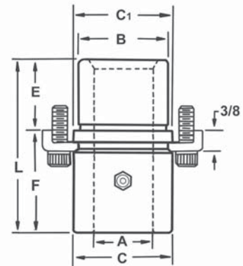
STANDARD SHOULDER
